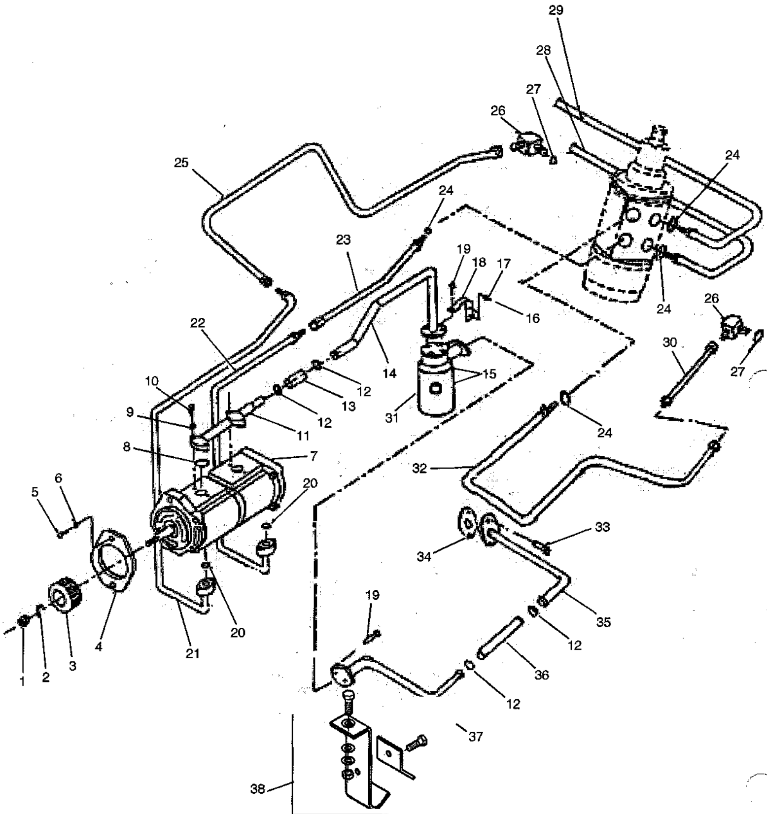
HYDRAULIC PUMP (TANDEM) - 535
