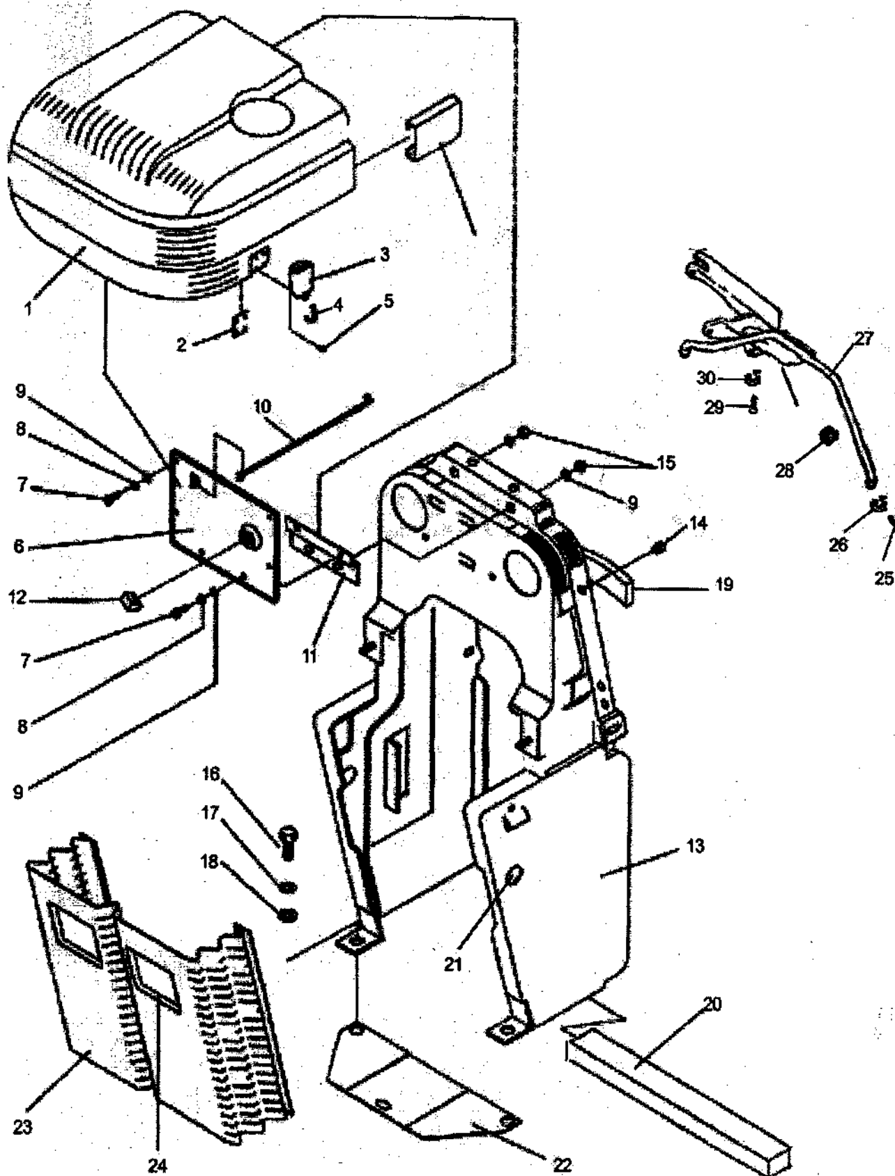
RADIATOR SHELL
