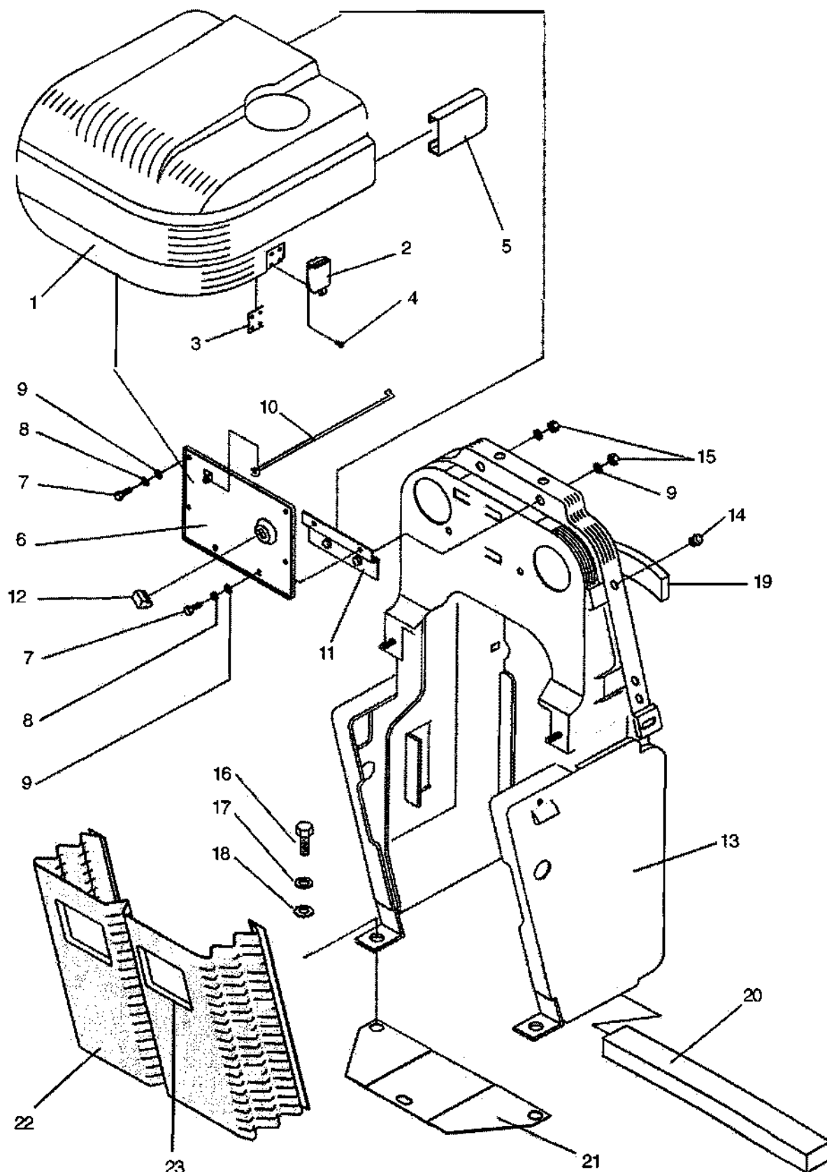
RADIATOR SHELL
