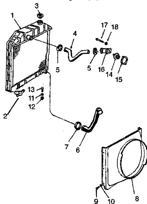
RADIATOR
