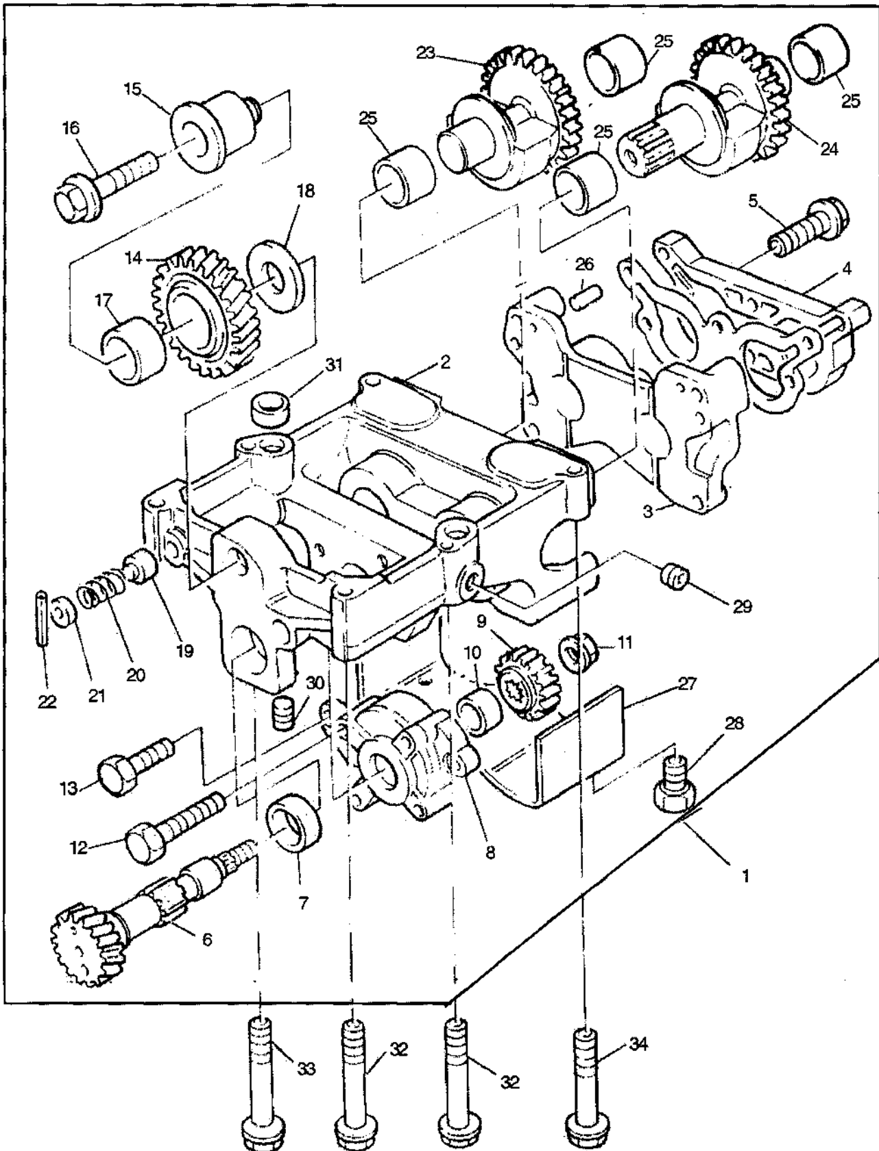
BALANCER UNIT
