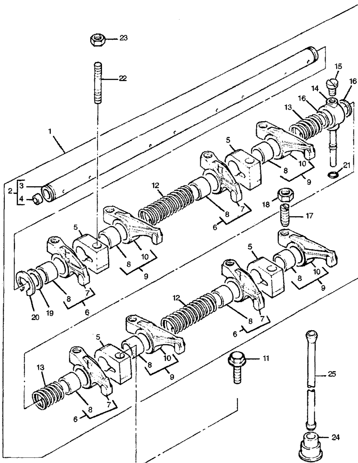
ROCKER SHAFT
